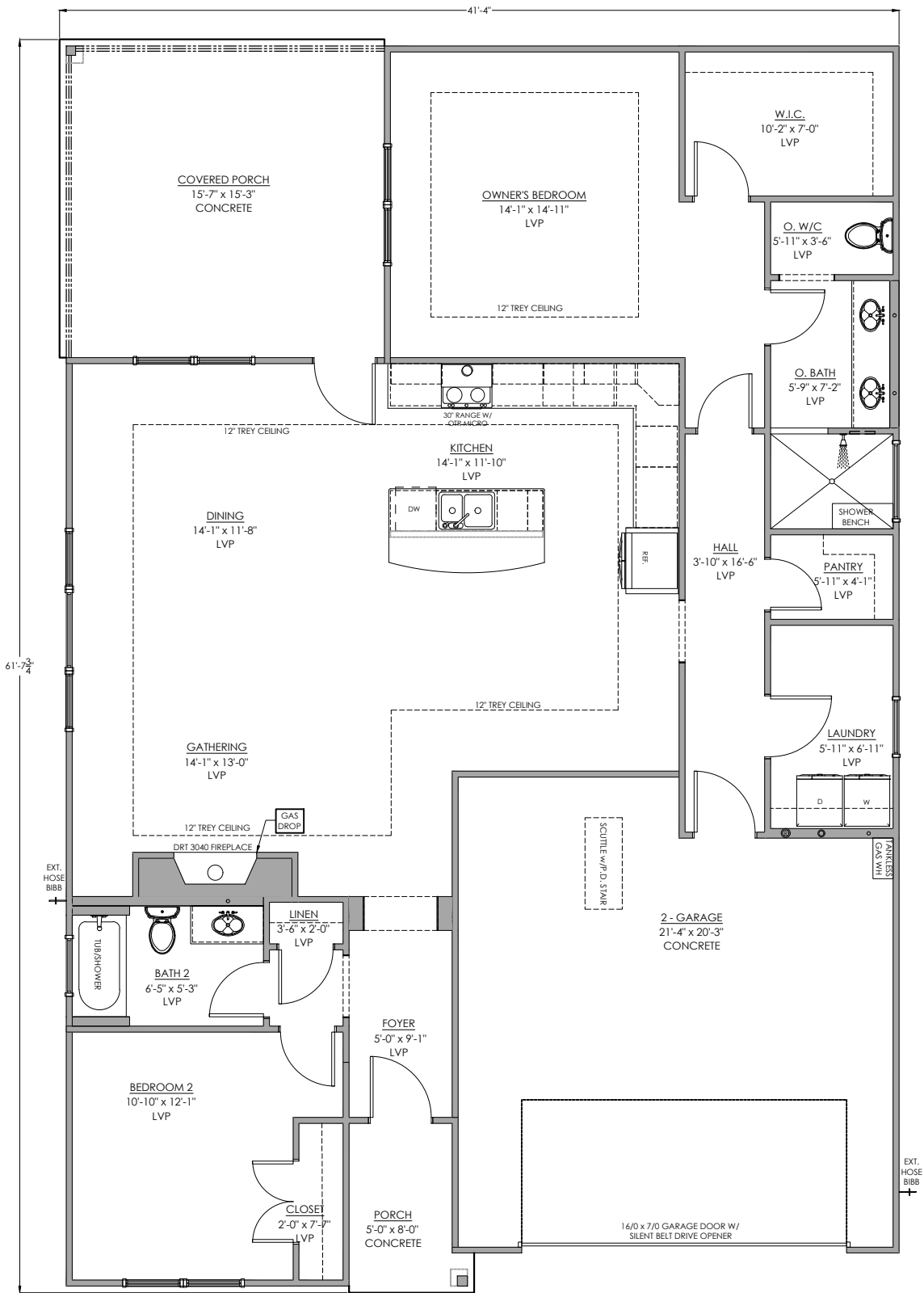
Main Floor Plan 1741 SF
