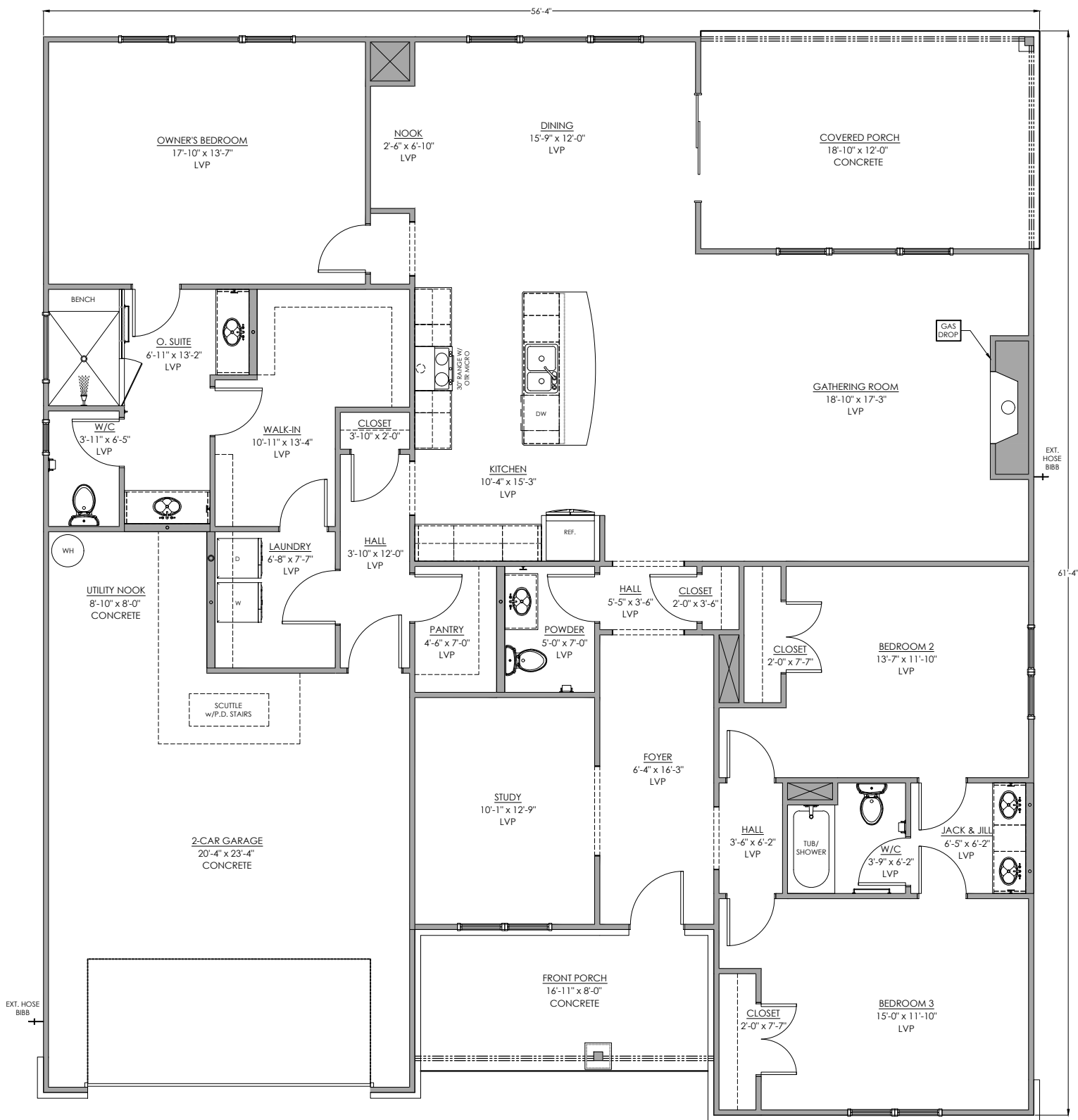
Main Floor Plan 2466 SF
