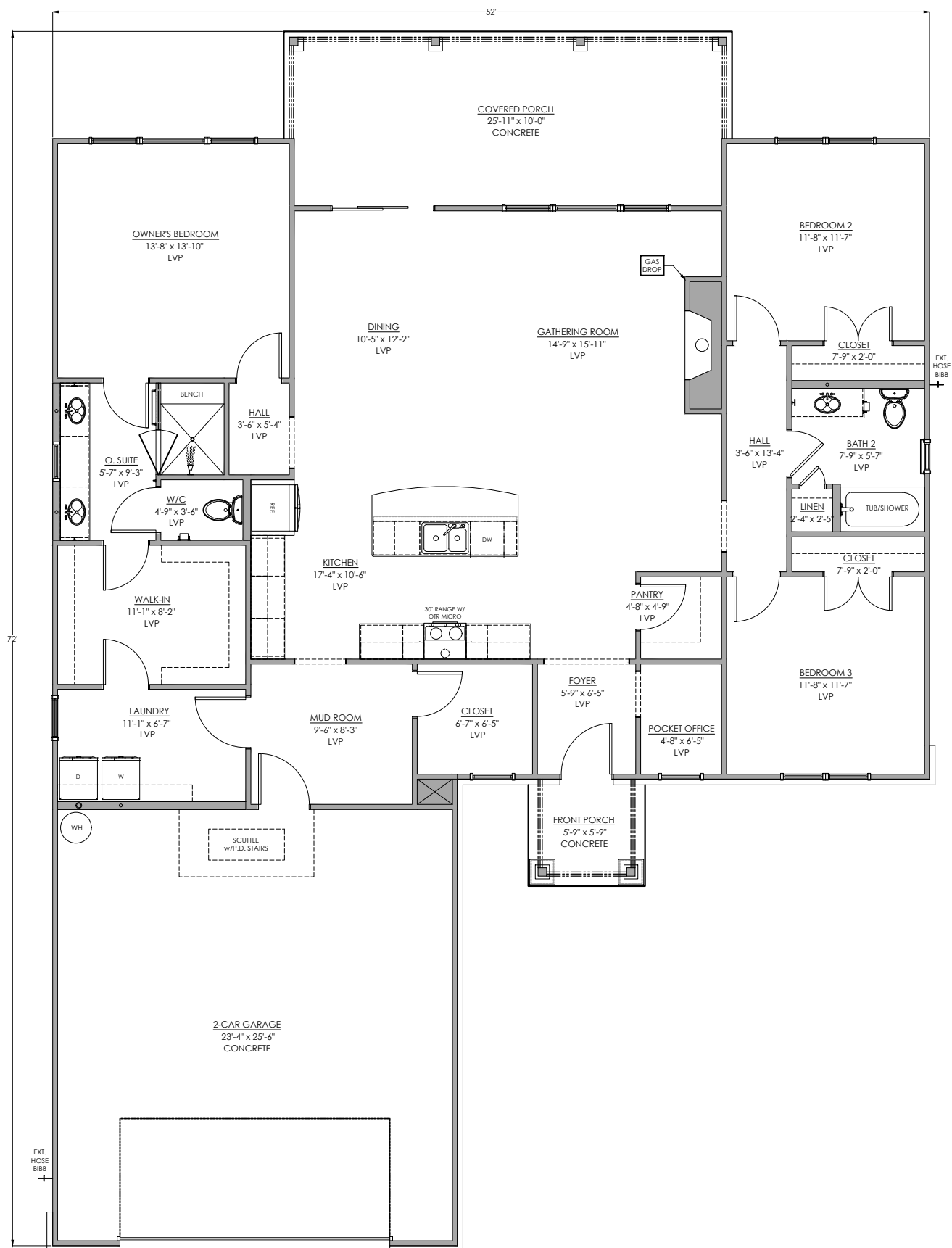
Main Floor Plan 1956 SF
