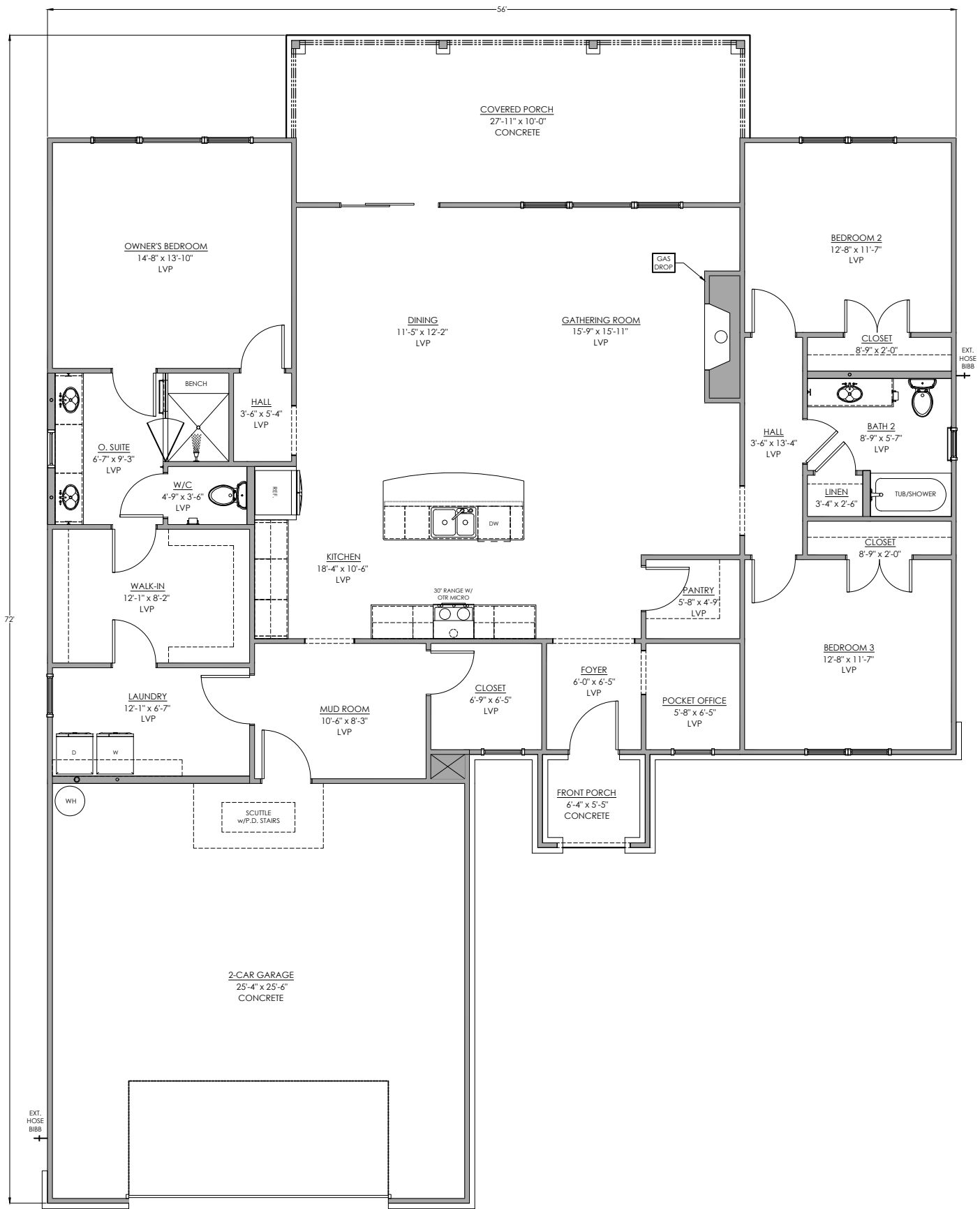
Main Floor Plan 2106 SF
