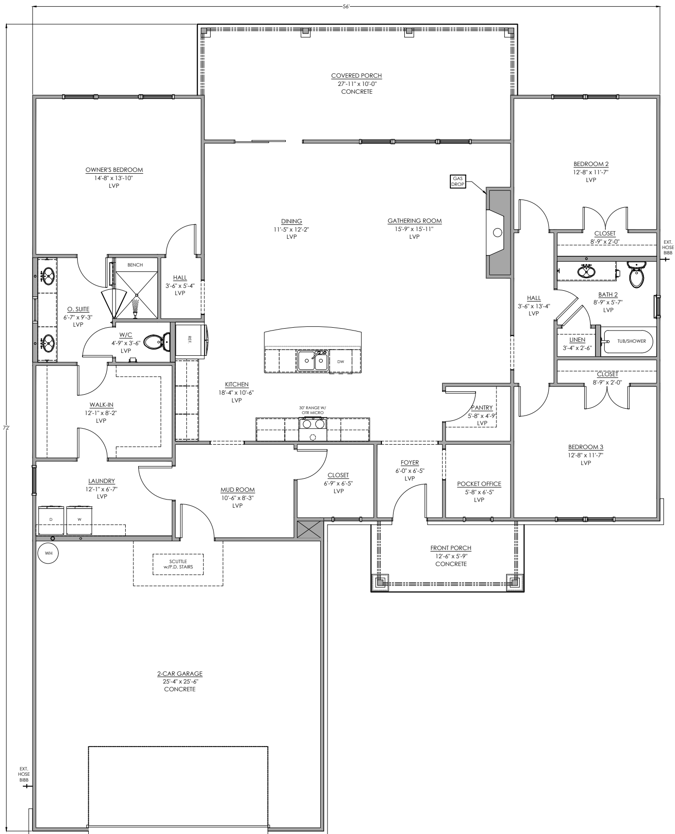
Main Floor Plan 2106 SF
