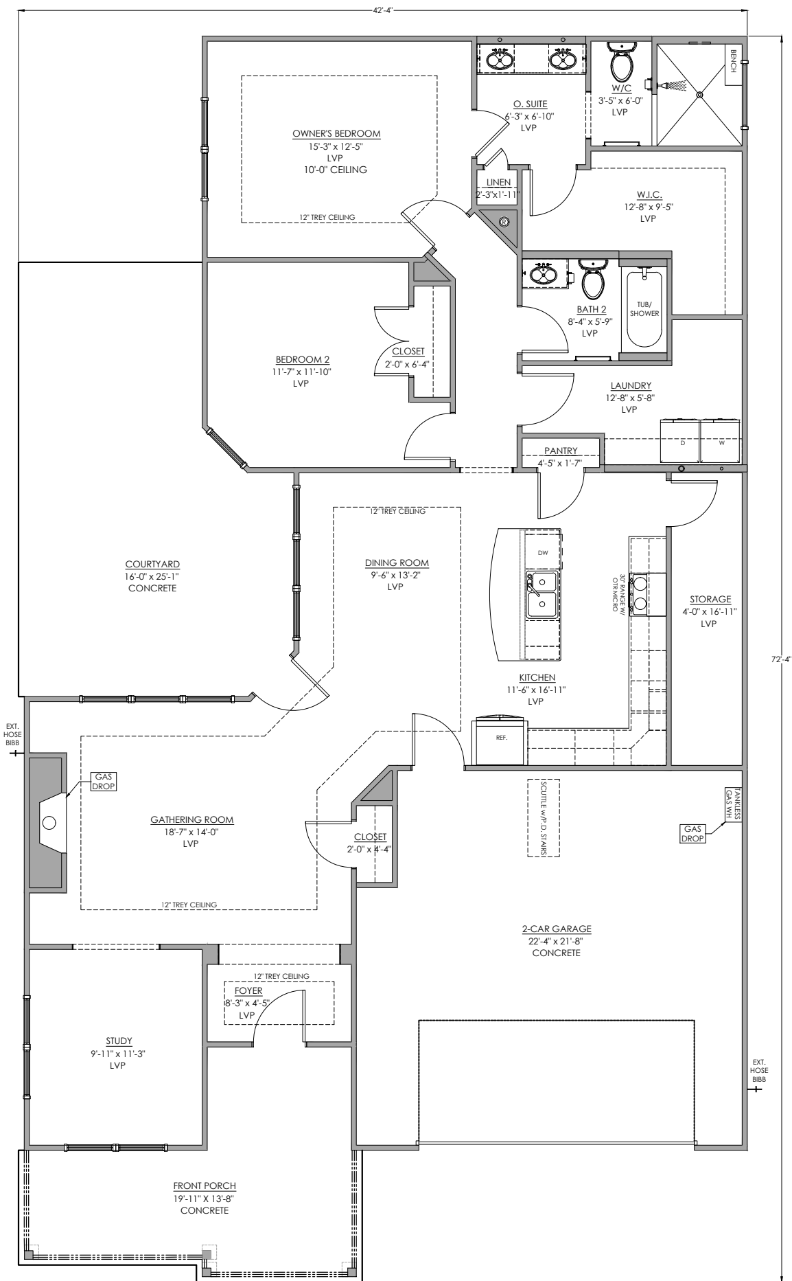
Main Floor Plan 1748 SF
