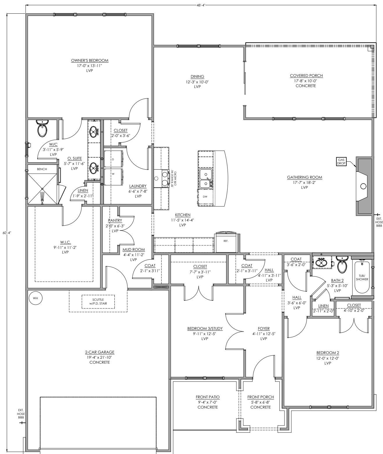
Main Floor Plan 1955 SF
