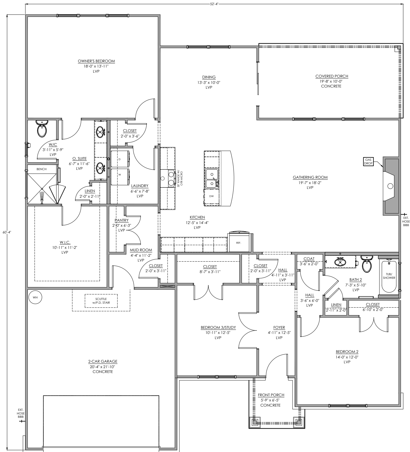
Main Floor Plan 2123 SF
