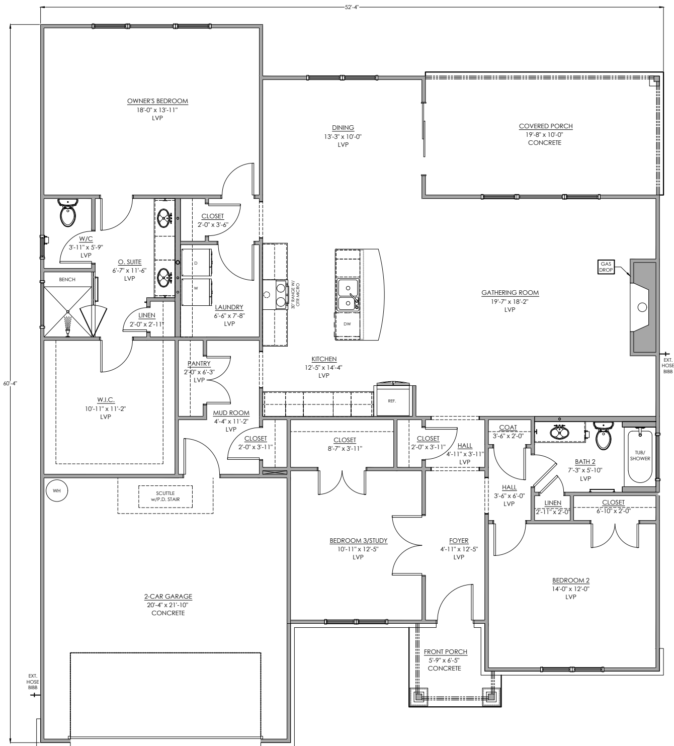
Main Floor Plan 2123 SF
