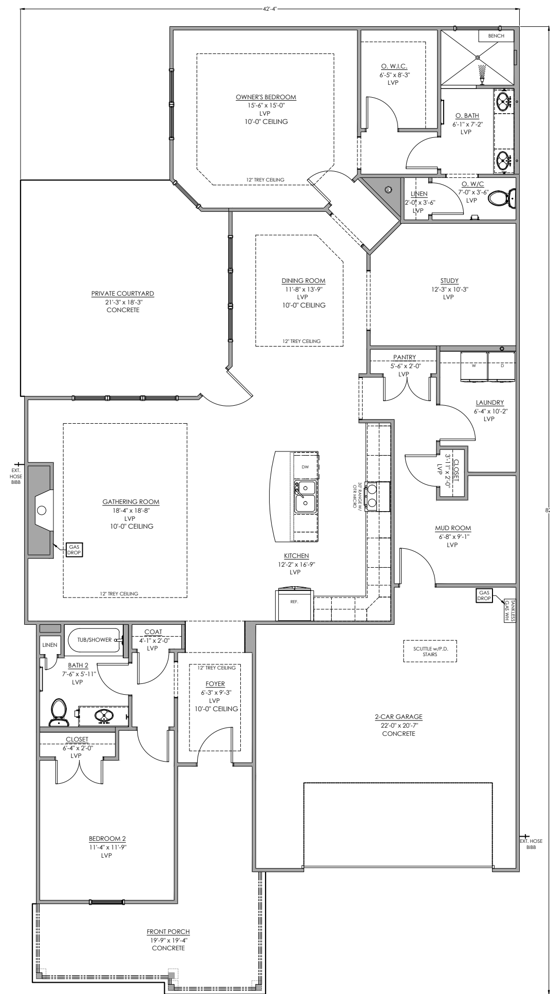
Main Floor Plan 2033 SF
