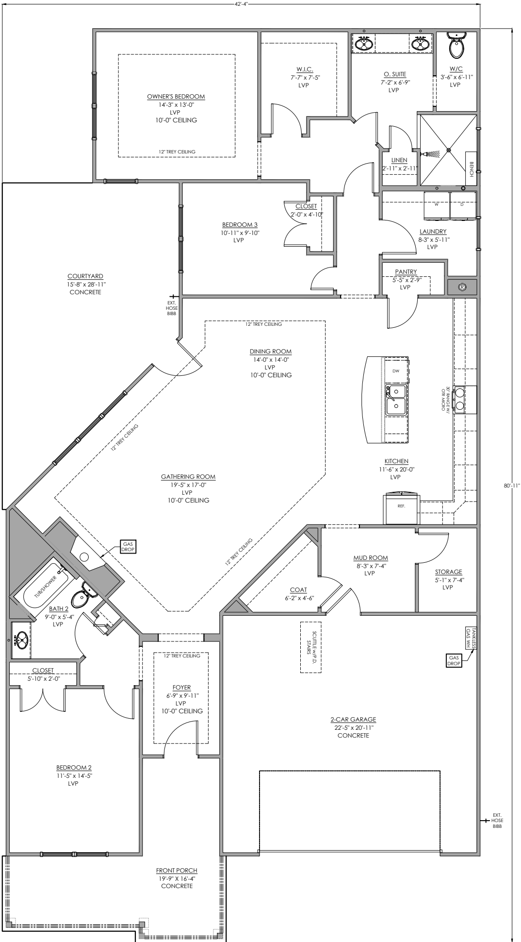
Main Floor Plan 2140 SF
