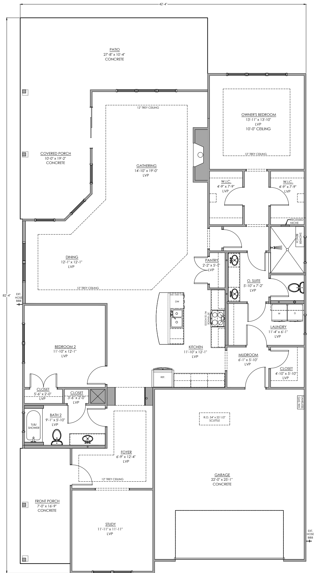
Main Floor Plan 2161 SF
