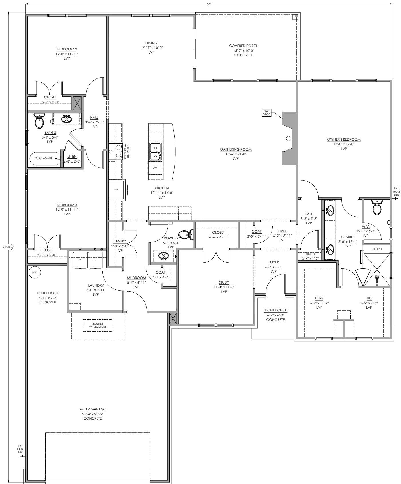
Main Floor Plan 2326 SF
