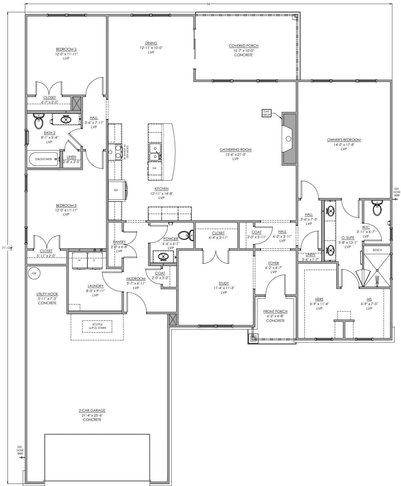
Main Floor Plan 2326 SF
