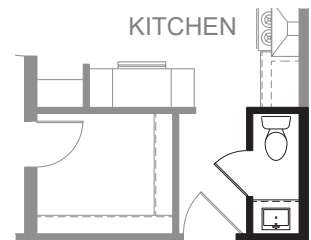
HALF BATH OPTION
