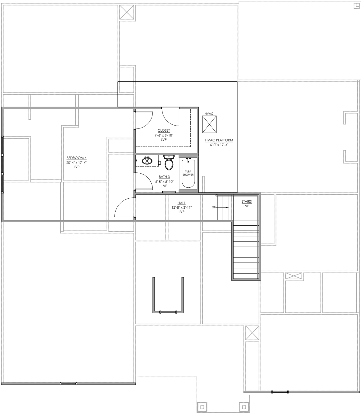
Second Floor Plan 580 SF
