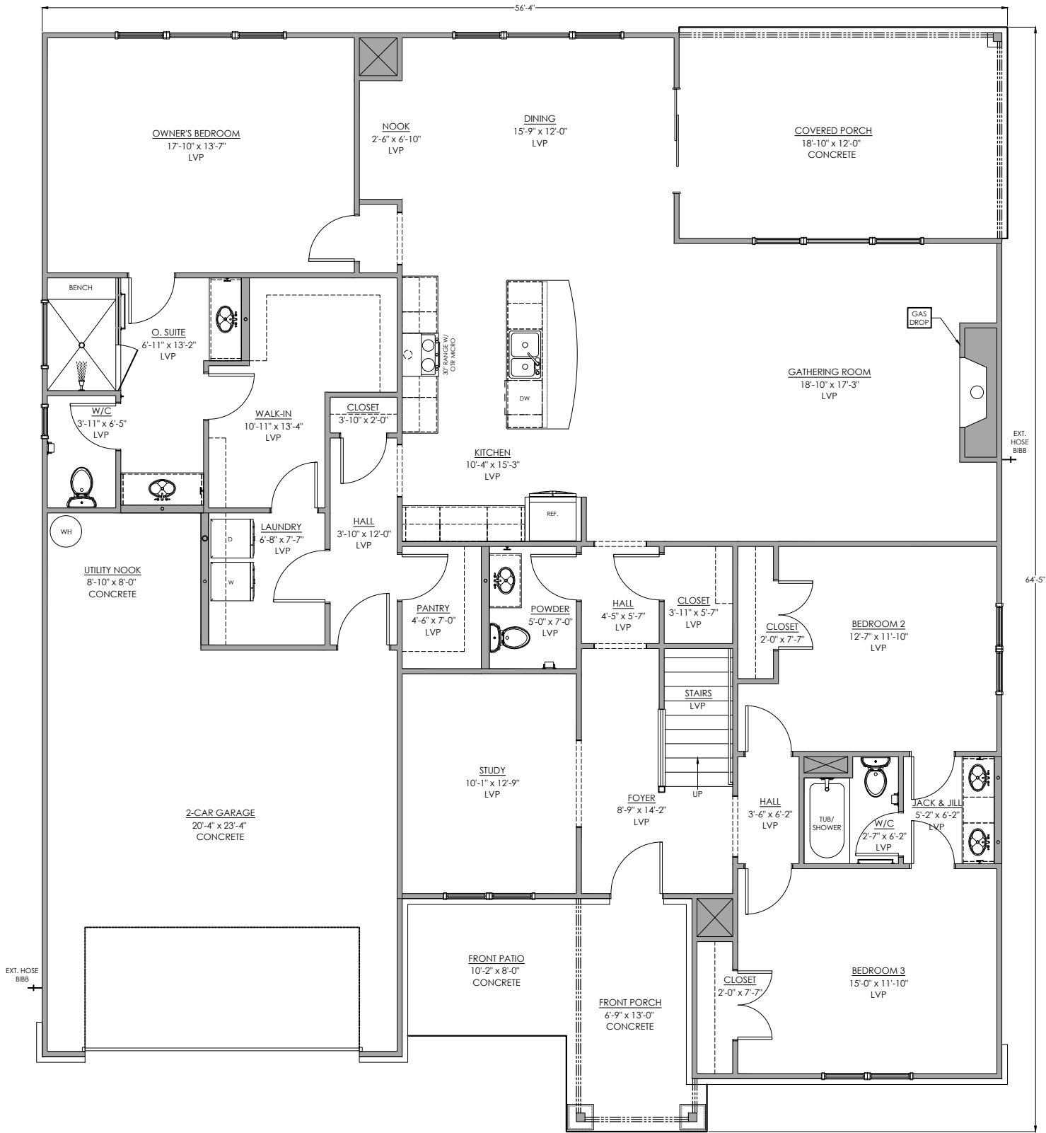
Main Floor Plan 2466 SF
