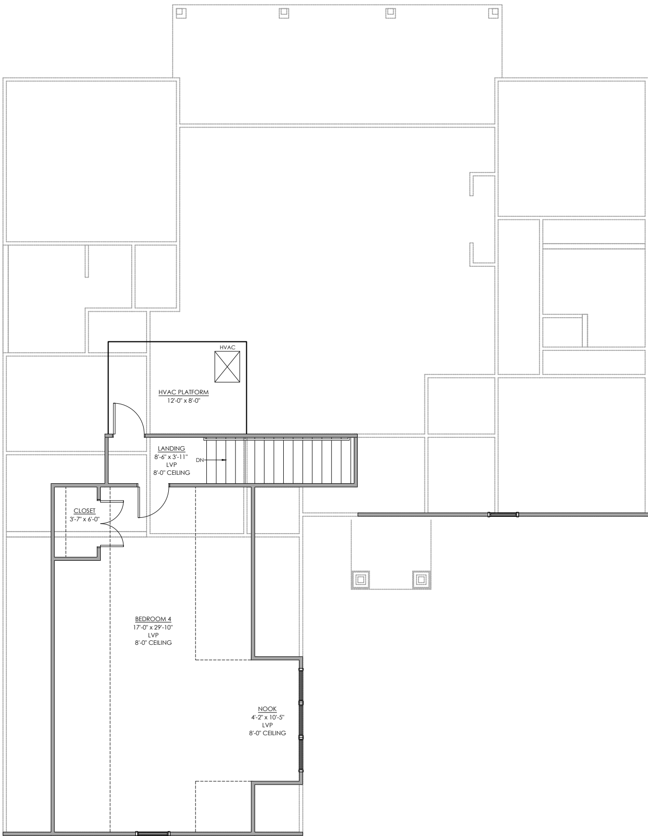
Second Floor Plan 696 SF
