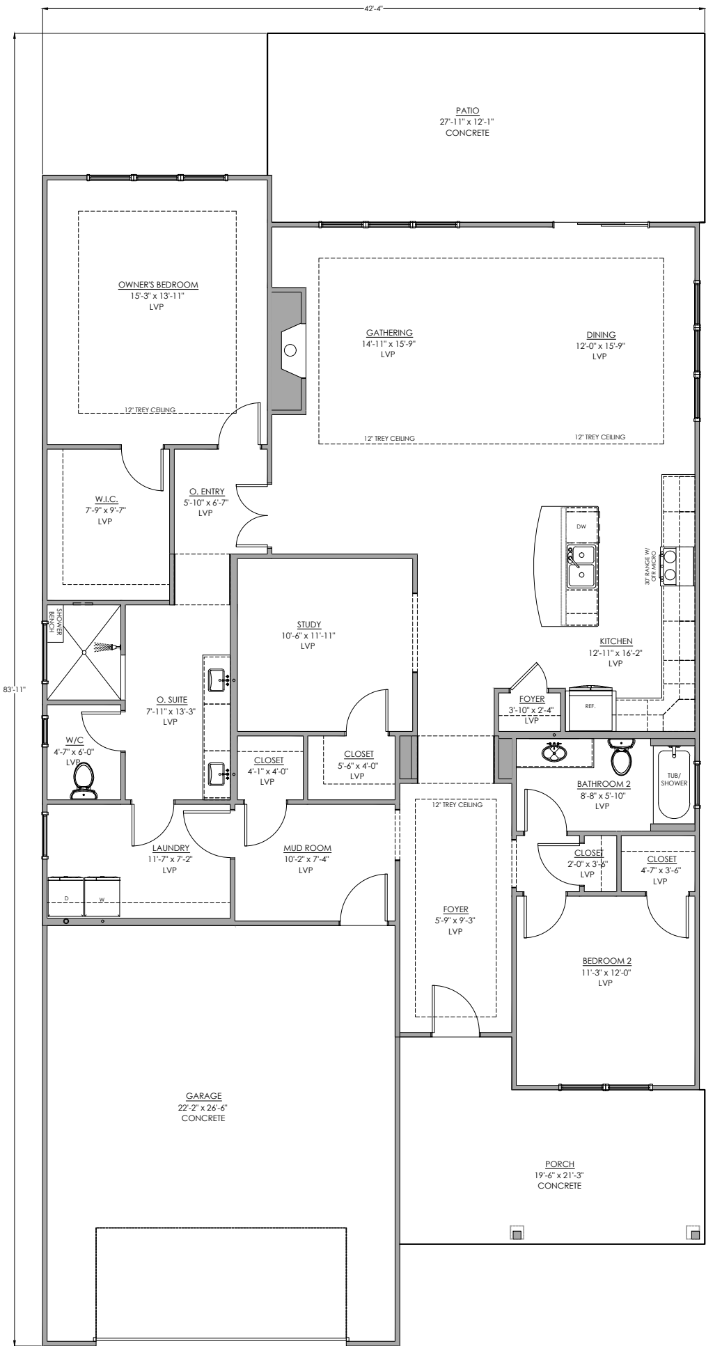
Main Floor Plan 2153 SF
