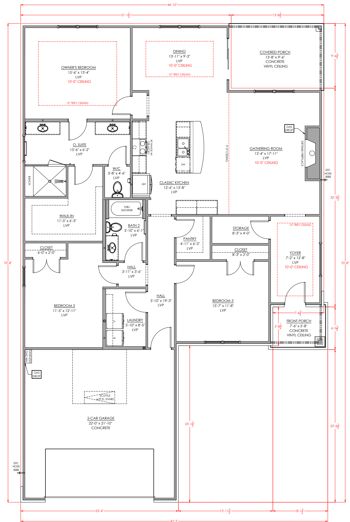
Main Floor Plan 1955 SF
