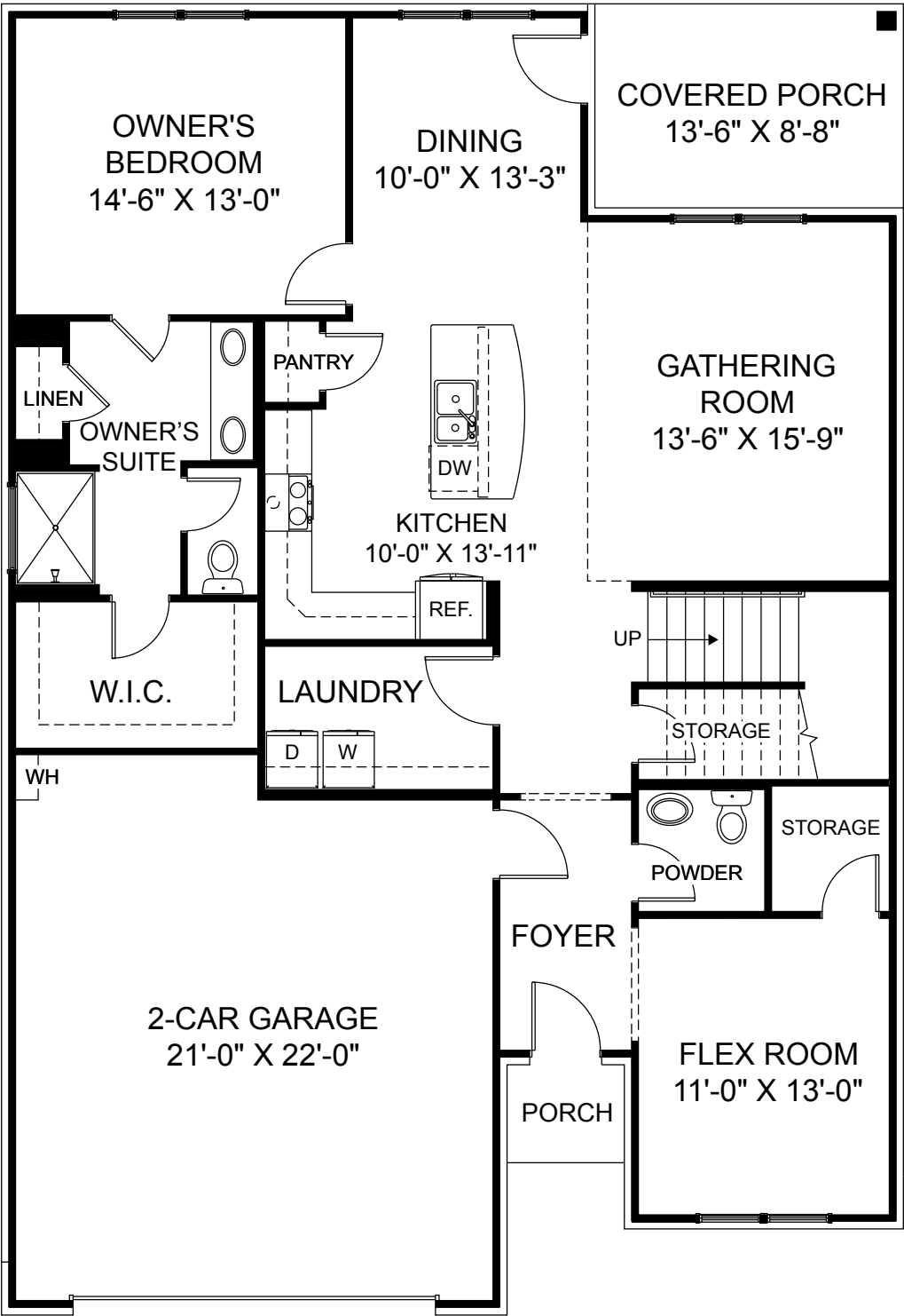
First Floor
