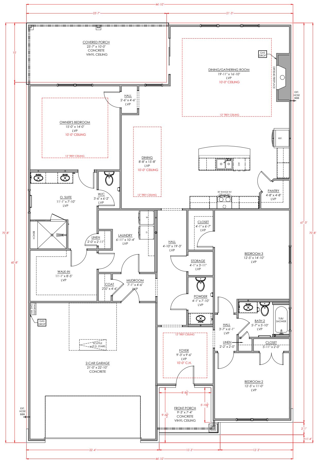
Main Floor Plan 2270 SF
