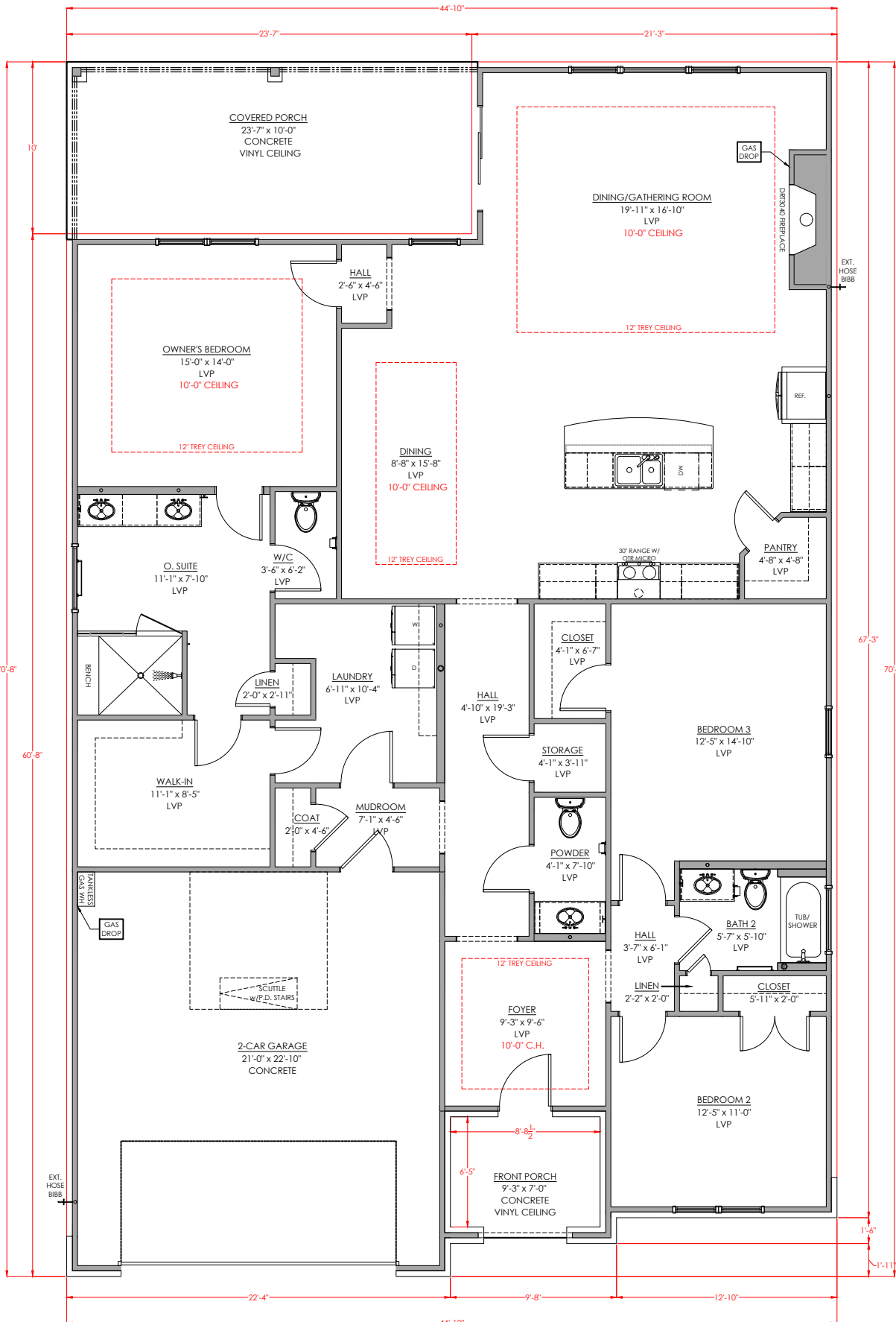
Main Floor Plan 2270 SF
