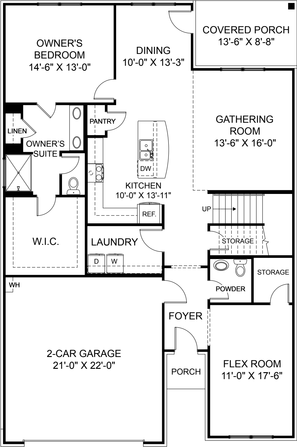
First Floor
