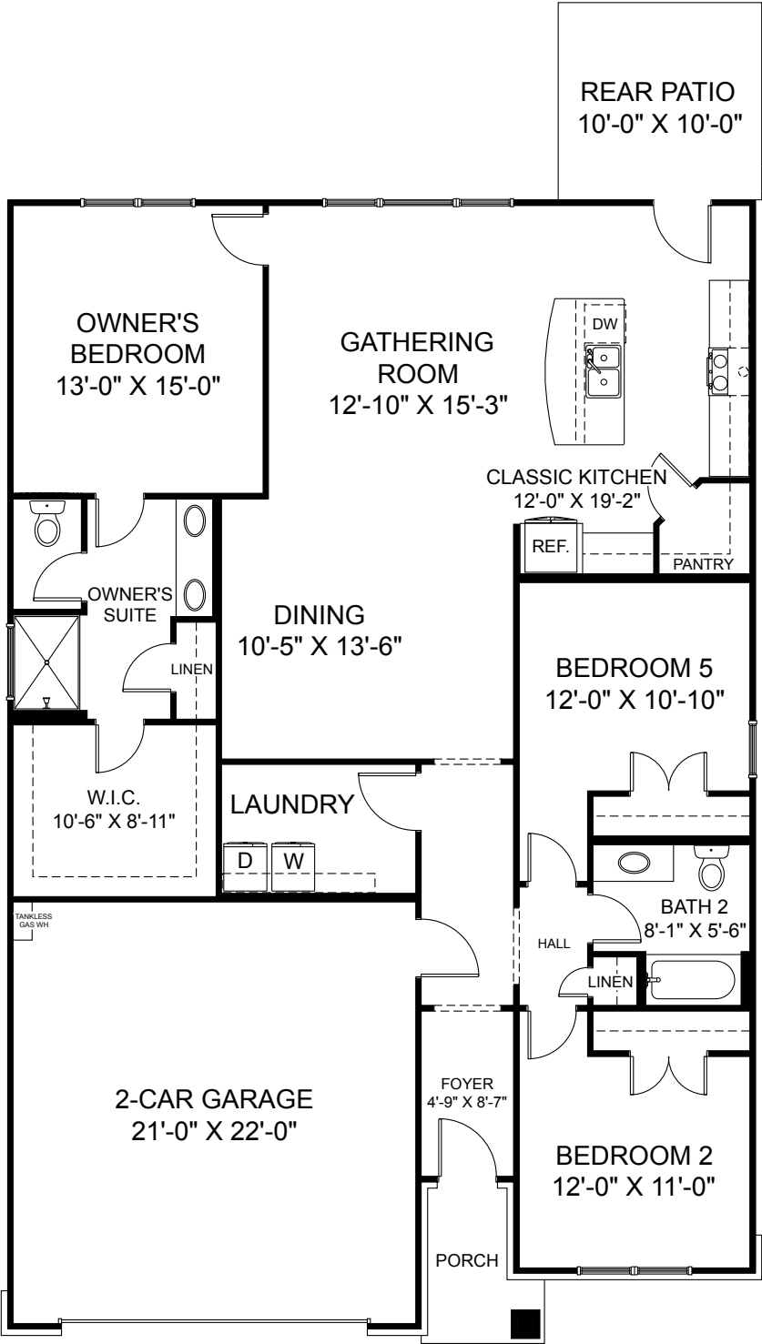
Floor Plan
