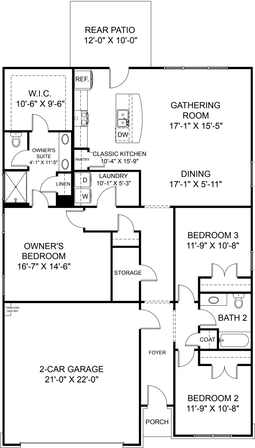
Floor Plan
